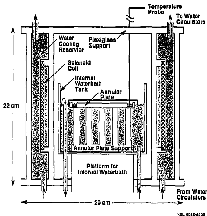
Fig. 1. Solenoidal cell culture exposure system. A uniform magnetic field is established in the center volume of a water-cooled solenoid ( n = 400 , 2.3 \Omega , 20.1 mH ) where a specialized multi-ring annular cell-culture plate is positioned. The cell-culture plate is isolated from the solenoid, vibration-free, and temperature-regulated to 37 \pm 0.05^\circ C .
