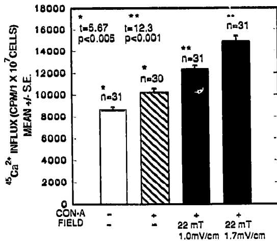
Fig. 4. Induced electric field dependence of calcium influx in activated thymocytes. Cells were exposed in a solenoid to a uniform, 60 Hz, 22 mT magnetic field and simultaneously to E_{\text{induced}} of either 1.0 mV/cm (middle well) or 1.7 mV/cm (outer well): 1 \mu g/ml Con A, 37 \pm 0.05°C, 60 min. Data subjected to a one-tailed t -test: * t = 5.67 , P < 0.005 , df = 59 for a comparison of resting to Con A-activated thymocytes (no field); ** t = 12.3 , P < 0.001 , df = 60 for a comparison of 1.0 to 1.7 mV/cm electric field treatment of Con A-activated thymocytes.
